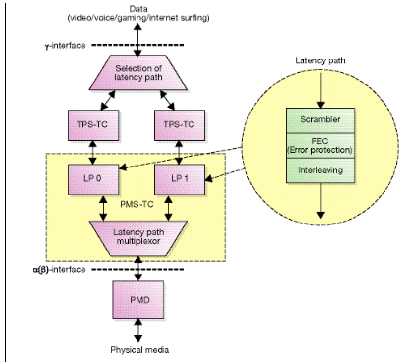
Figure 13 Reference model of the transceiver. The dotted lines indicate an optional latency path.
