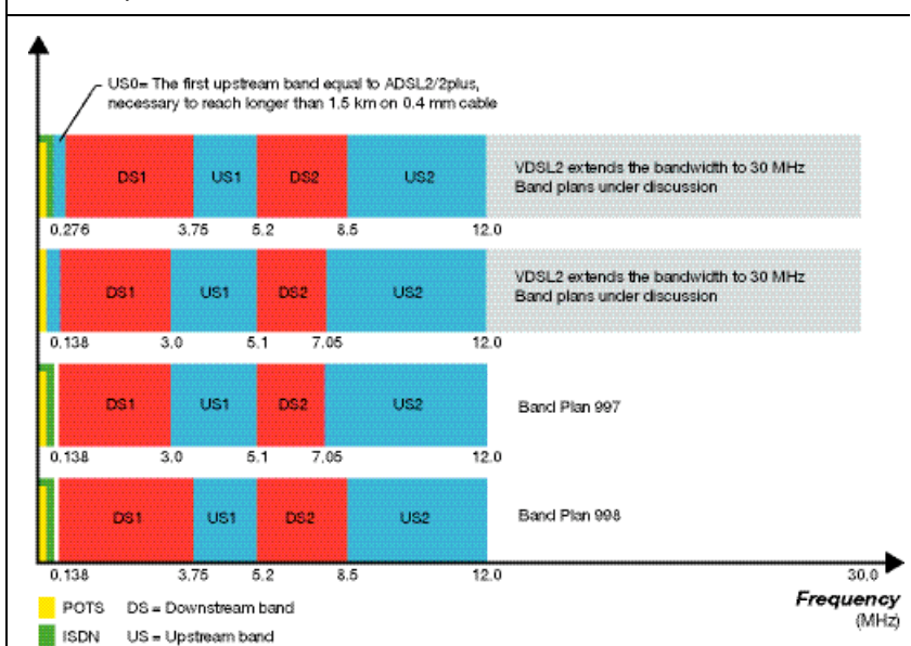
Figure 5 The band plans of VDSL1 and VDSL2.
