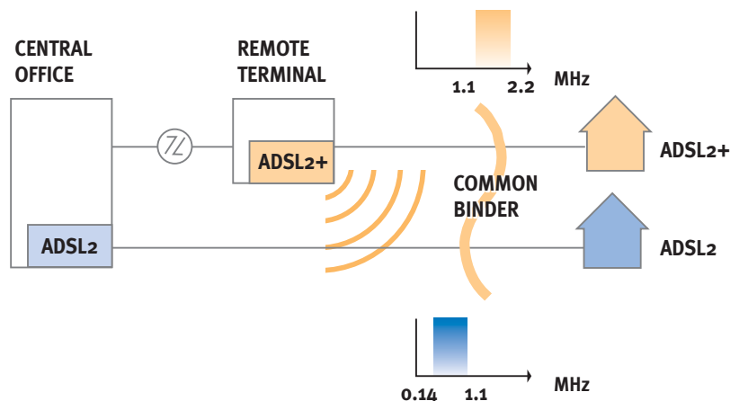
FIGURE 10: ADSL2+ CAN BE USED TO REDUCE CROSSTALK.
