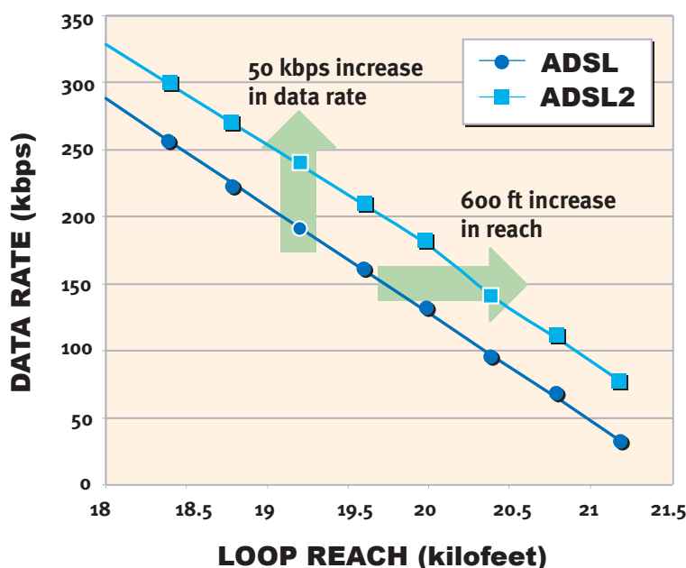
FIGURE 2: ADSL2 SYSTEMS CAN DELIVER AN IMPROVEMENT IN REACH OF ABOUT 600 FEET.
