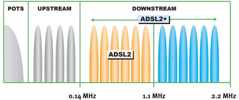
FIGURE 8: ADSL2+ DOUBLES THE BANDWIDTH USED TO CARRY DATA.
