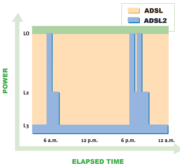
FIGURE 3: ADSL2'S L2 POWER MODE ALLOWS A BROADBAND MODEM TO QUICKLY MOVE FROM L2 TO L0 OPERATION AND BACK WITHOUT BIT ERRORS.
