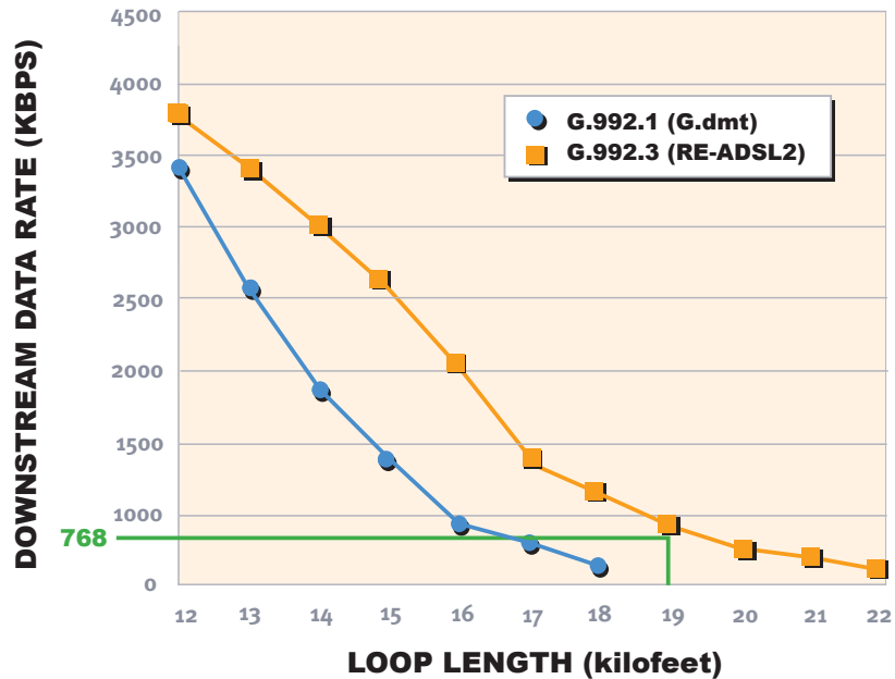
FIGURE 12: REACH EXTENDED ADSL2 (RE-ADSL2) REACH IMPROVEMENT
