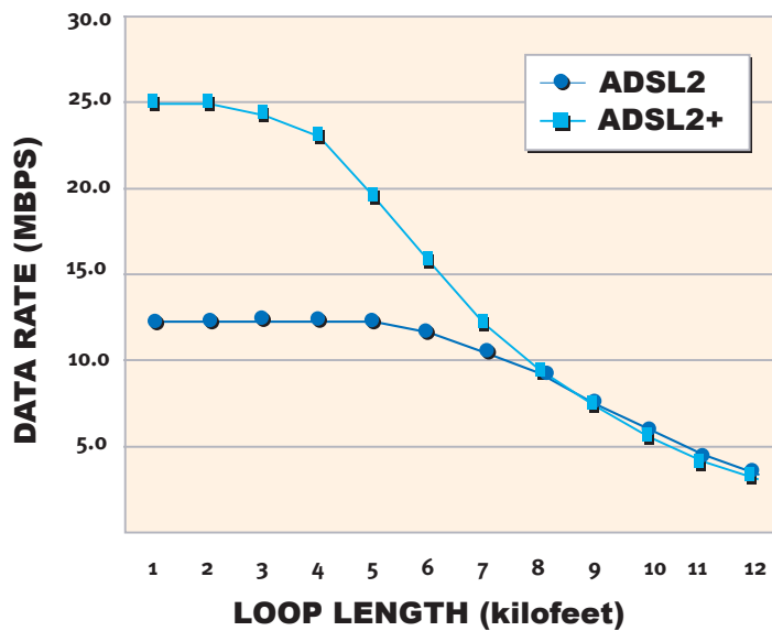
FIGURE 9: ADSL2+ DOUBLES THE MAXIMUM DATA RATE.
