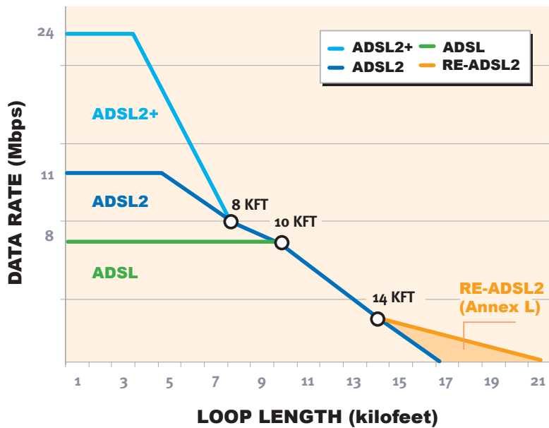
FIGURE 14: RATE & REACH PERFORMANCE OF ADSL AND ADSL2 STANDARDS
