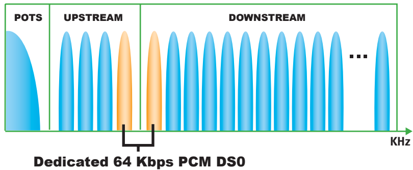
FIGURE 6: CVoDSL DEDICATES CHANNELS OF PHYSICAL LAYER BANDWIDTH TO CARRY TDM VOICE LINES.
